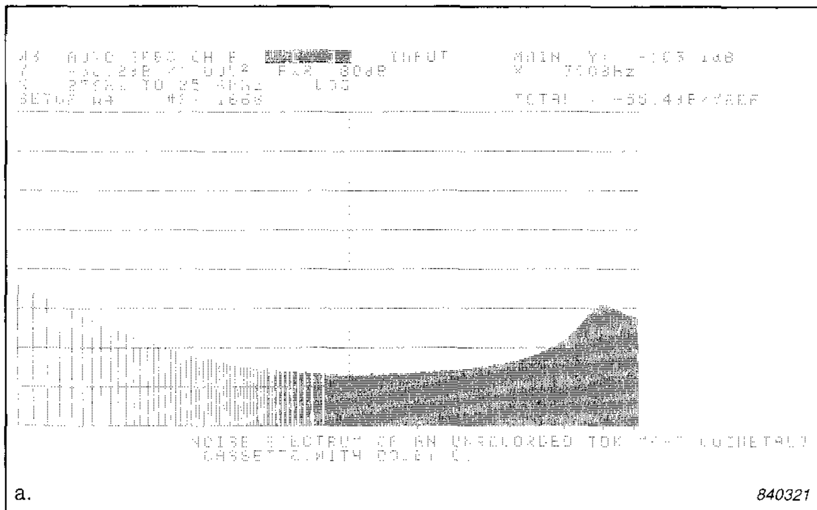
Fig. 18. (a) The noise spectrum of a factory bulk-erased tape replayed with Dolby C noise reduction system. Shown here with logarithmic frequency axis. The total noise power can be read out in the "TOTAL" field
